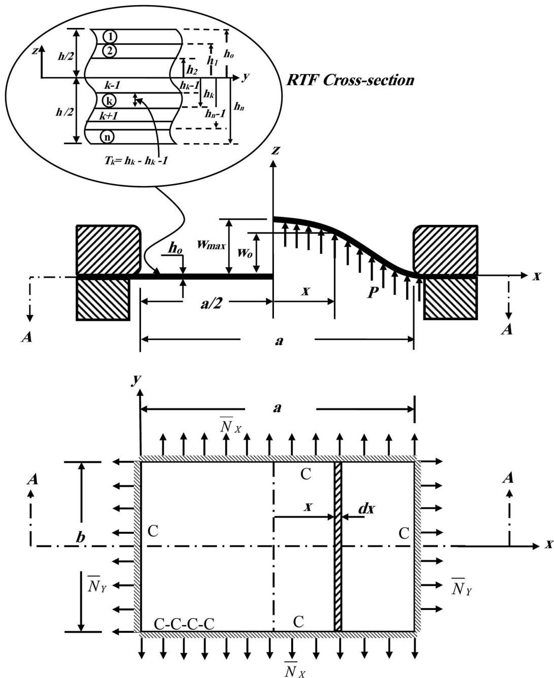
Figure 3. The geometrical model of the bulge test for the BFRP composite NRD subjected to in-plane (pre-stressed) load \overline{N}_x and \overline{N}_y with clamped edges (CCCC).
