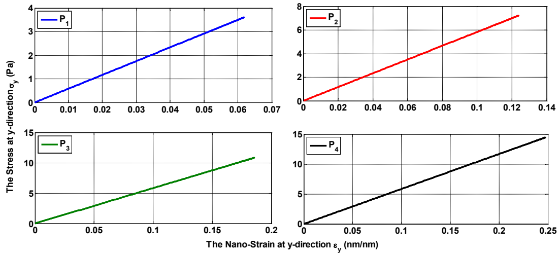
Figure 13. Stress and Nano-strain relationship at y-direction with differential pressure of NRD for BFRP composite material with [0^\circ/90^\circ/0^\circ/90^\circ/0^\circ]_s laminate layer angle.
