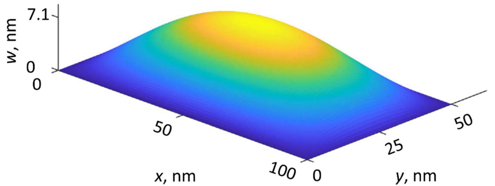
Figure 15. The diaphragm 3D deformation.
