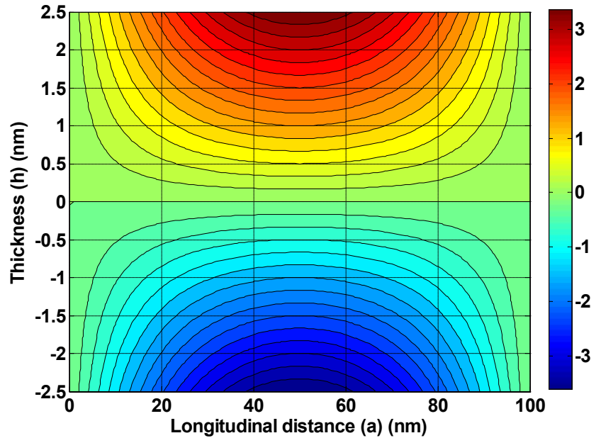
Figure 10. The stress distribution across the NRD thickness in the contour profile.
