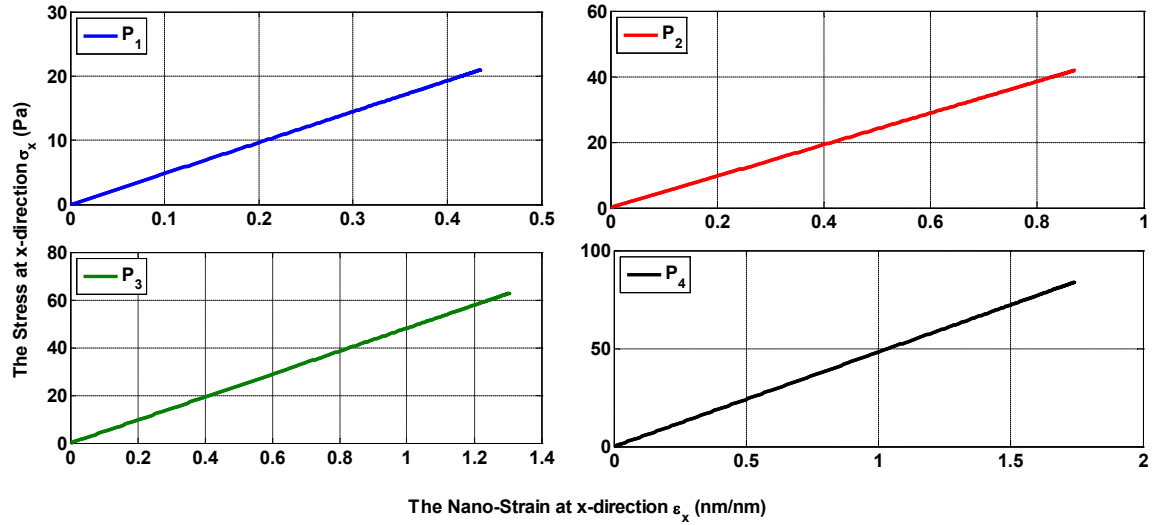
Figure 12. Stress and Nano-strain relationship at x-direction with differential pressure of NRD for BFRP composite material with [0^\circ/90^\circ/0^\circ/90^\circ/0^\circ]_s laminate layer angle.
