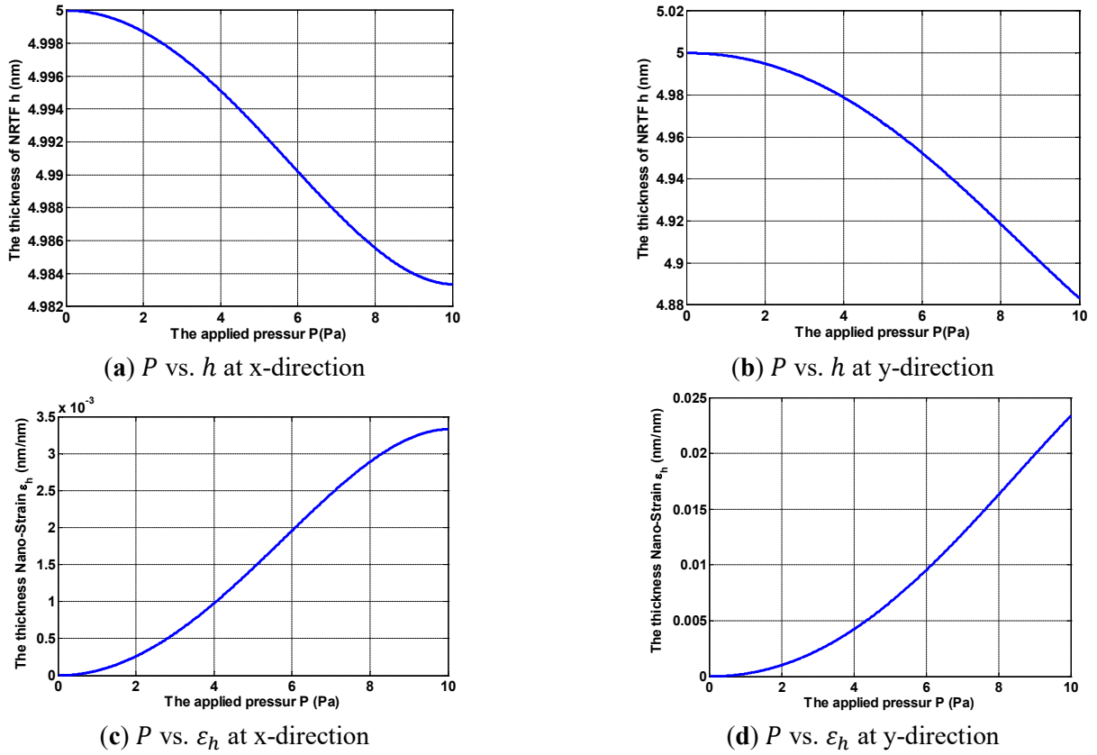
Figure 14. The relation between differential pressure ( P ) and the thickness nano-deformation of NRD for the BFRP composite material with [0^\circ/90^\circ/0^\circ/90^\circ/0^\circ]_S laminate layer angle.
