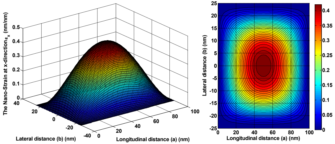
Figure 7. Nano-strain \varepsilon_x (nm/nm) distribution along NRD for the BFRP composite material with [0^\circ/90^\circ/0^\circ/90^\circ/0^\circ]_S laminate layer angle, contour profile at right and 3D profile at left.
