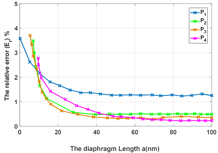
Figure 16. The relative error ( E_r ) between analytical and numerical results under various pressures ( P ).
