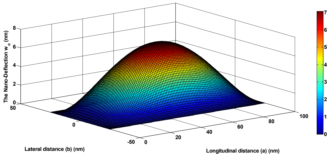
Figure 6. The 3D Nano-deflection distribution along NRD for BFRP composite material with [0^\circ/90^\circ/0^\circ/90^\circ/0^\circ]_S laminate layer angle.
