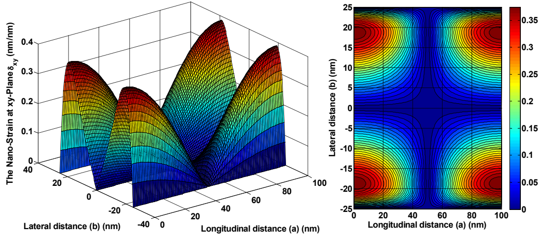
Figure 9. Nano-strain \gamma_{xy} (nm/nm) distribution along NRD for the BFRP composite material with [0^\circ/90^\circ/0^\circ/90^\circ/0^\circ]_5 laminate layer angle, contour profile at right and 3D profile at left.
