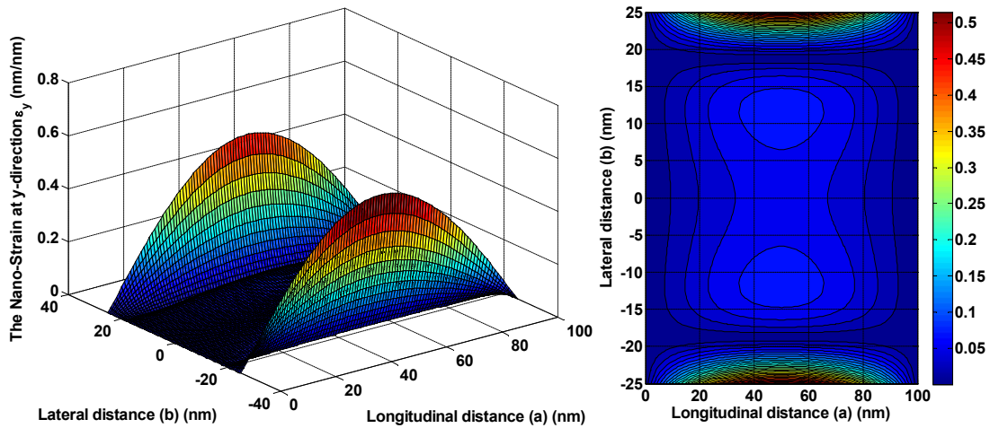
Figure 8. Nano-strain \varepsilon_y (nm/nm) distribution along NRD for the BFRP composite material with [0^\circ/90^\circ/0^\circ/90^\circ/0^\circ]_S laminate layer angle, contour profile at right and 3D profile at left.
