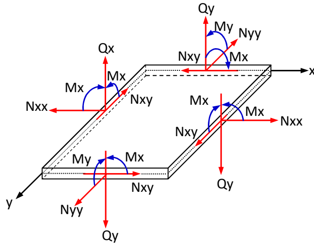
Figure 4. The shear forces and moments on a laminate.
