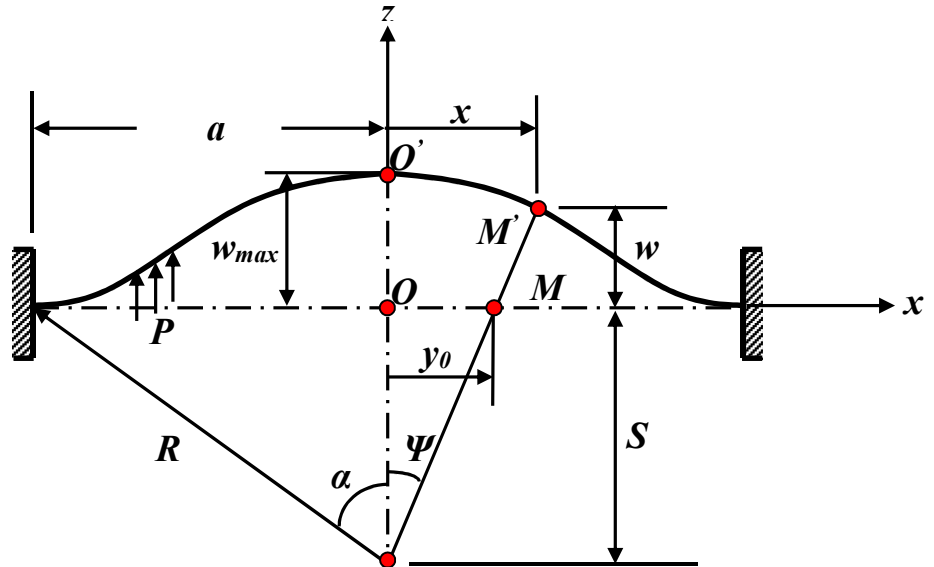
Figure 5. Schematic of deformation modeling.
